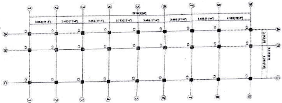
Column Layout Plan
