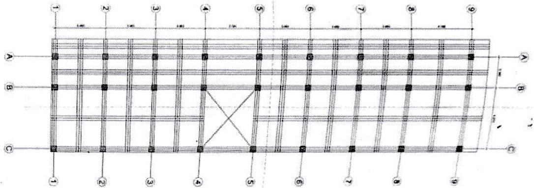
GROUND FLOOR SLAB REINFORCEMENT PLAN (BOTTOM BAR)
