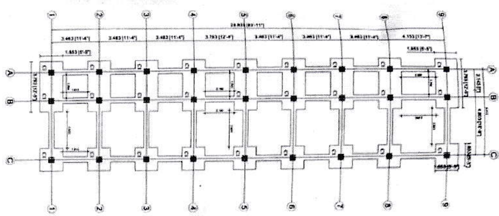
Trench Plan
