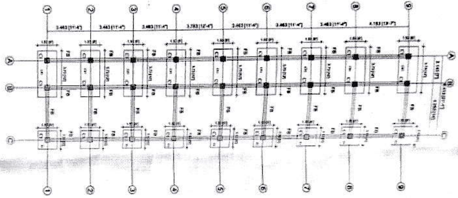
Foundation Layout Plan
