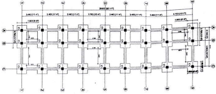
Trench Plan
