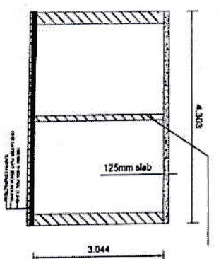
(B) Septic Tank Plan (C)
