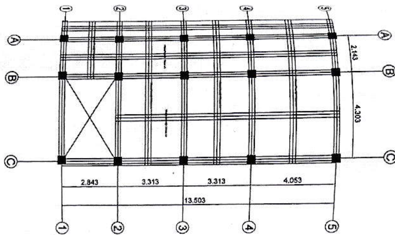
FIRST FLOOR SLAB REINFORCEMENT PLAN (BOTTOM BAR) SLAB THICKNESS : 125MM REF: 10 MM Ø @ 150 MM C/C
