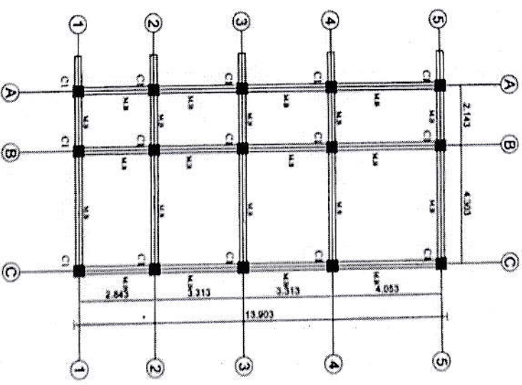
First Floor Beam Layout Plan
