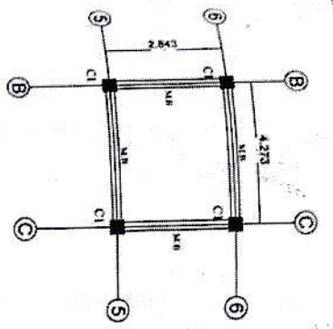
Second Floor Beam Layout Plan Main Beam (0.25*0.35)
