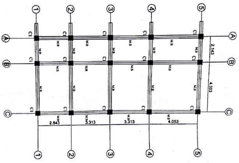
Ground Floor Beam Layout Plan
