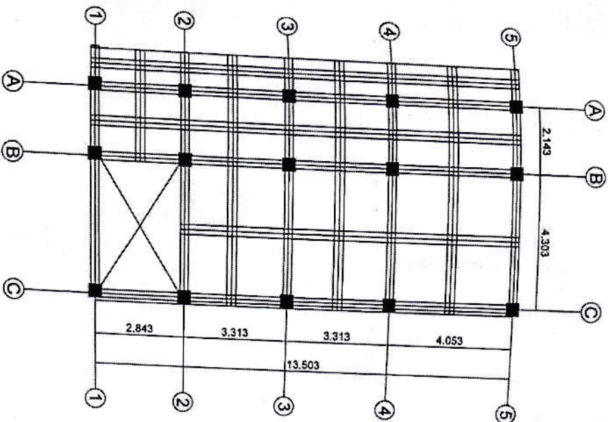
GROUND FLOOR SLAB REINFORCEMENT PLAN (BOTTOM BAR)
