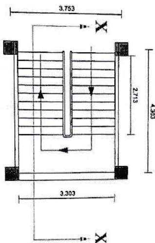
Staircase Plan
