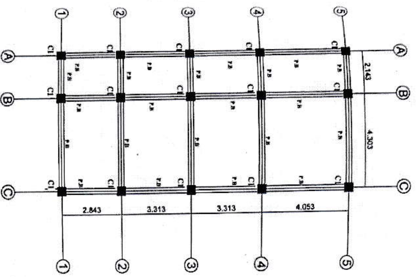
Plinth Beam Layout Plan
