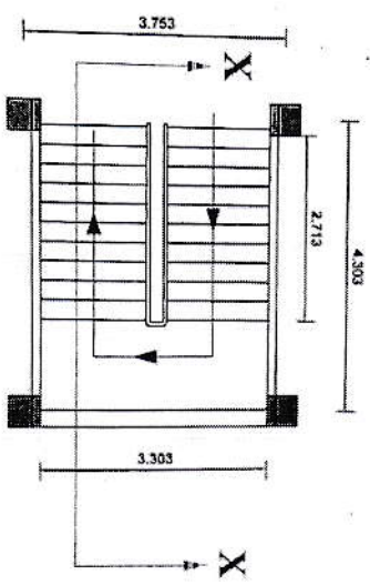
Staircase Plan
