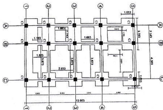
Trench Plan
