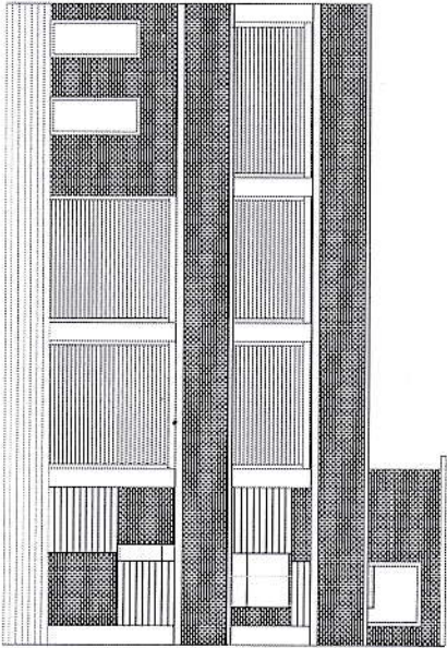
West Elevation
