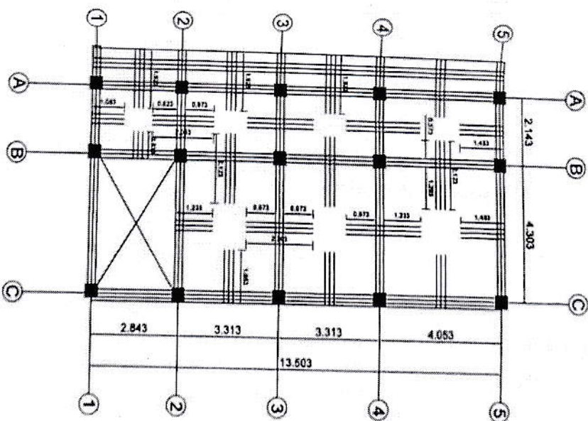
GROUND FLOOR SLAB REINFORCEMENT PLAN (TOP BAR)
