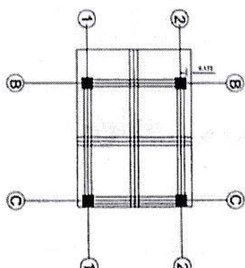
TOP FLOOR SLAB REINFORCEMENT PLAN (BOTTOM BAR) SLAB THICKNESS : 125MM REF: 10 MM Ø @ 150 MM C/C
