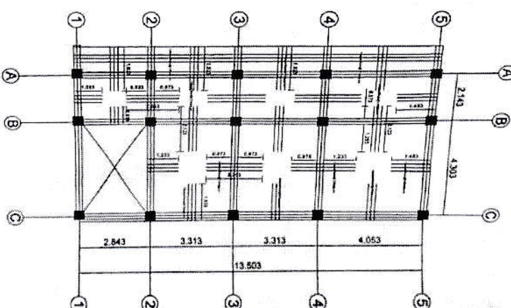
FIRST FLOOR SLAB REINFORCEMENT PLAN (TOP BAR) SLAB THICKNESS : 125MM REF: 10 MM Ø @ 150 MM C/C
