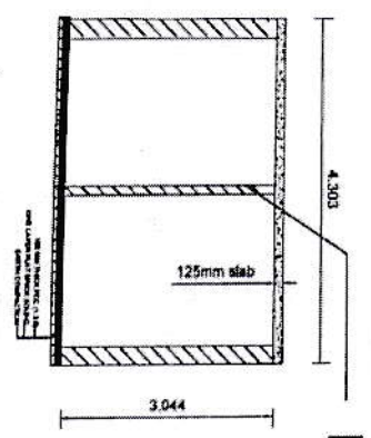
Septic Tank Plan
