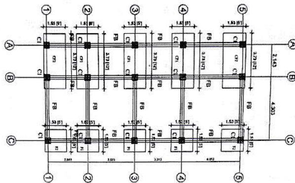
Foundation Layout Plan Foundation Beam: 0.25*0.3
